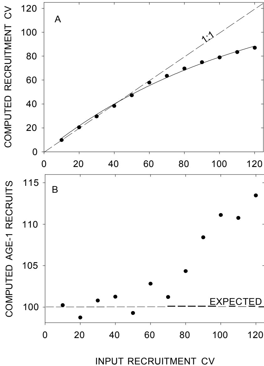
Figure 5-1. Input recruitment coefficients of variation (CV) entered in the Random (normally distributed) option in FAST plotted against the computed recruitment coefficients of variation for a 1,000 year simulation (A). Input recruitment CV's from the same option plotted against the average number of computed age-1 recruits for a 1,000 year simulation (B). The expected average number of age-1 recruits for each input recruitment CV was 100.
