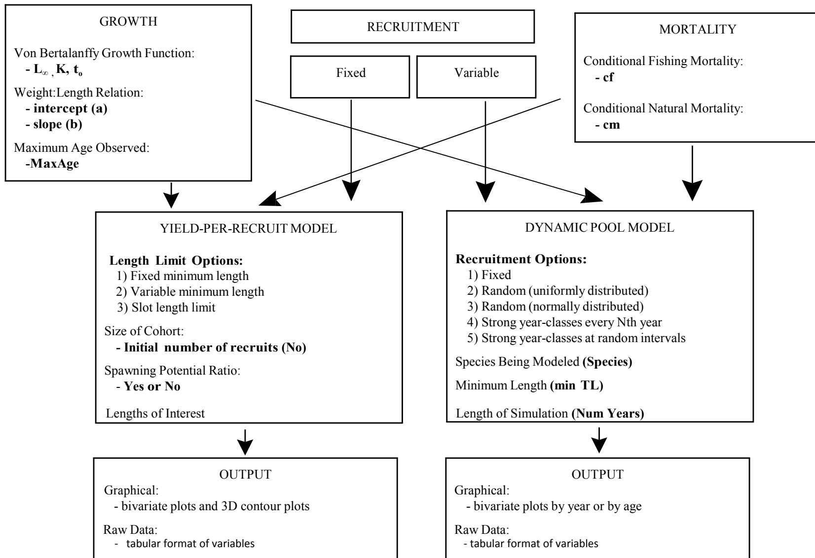
Figure 1-3. Schematic flow chart of the FAMS modeling program. Required input parameters are identified by bold print.
